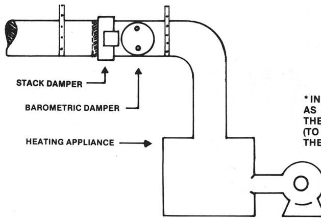
HORIZONTAL OR SLOPING INSTALLATION* Fig. 2
