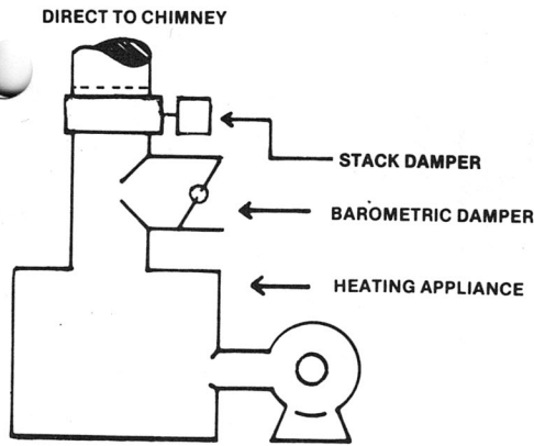
VERTICAL INSTALLATION Fig. 1
