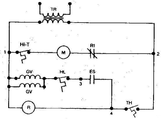
LADDER DIAGRAM
